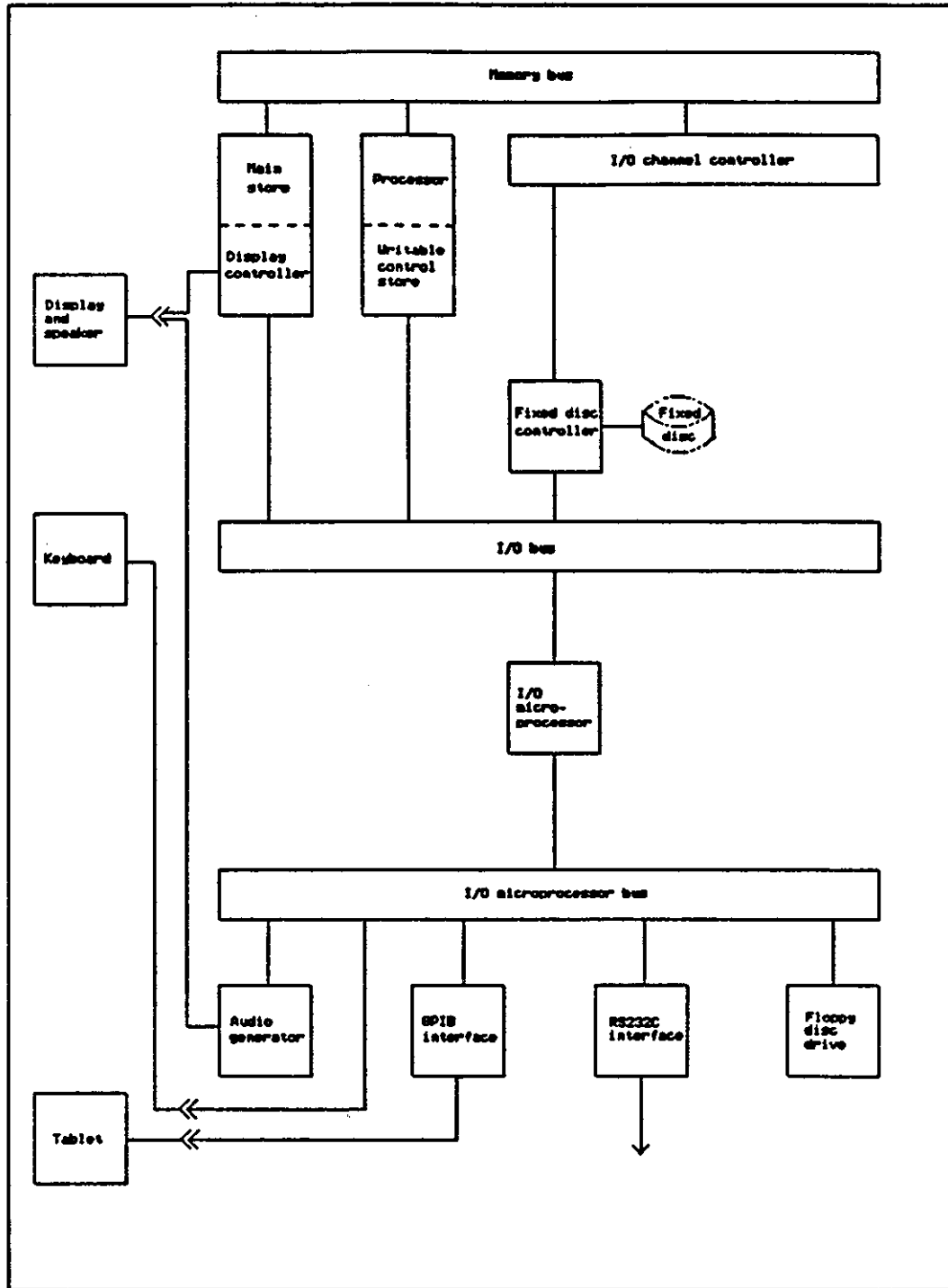
Figure 2-5 Components of Processor Box
