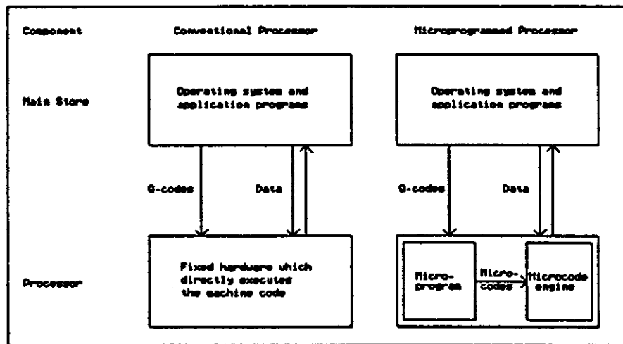
Figure 2-6 Microcode Executed by Microcode Engine
